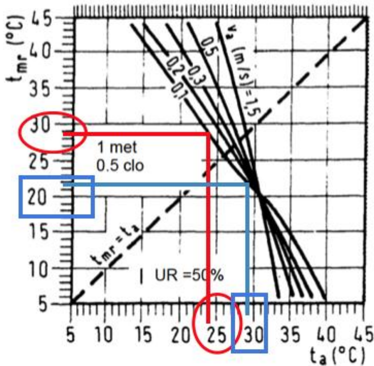
Fig. 3 - Curve isocomfort.
