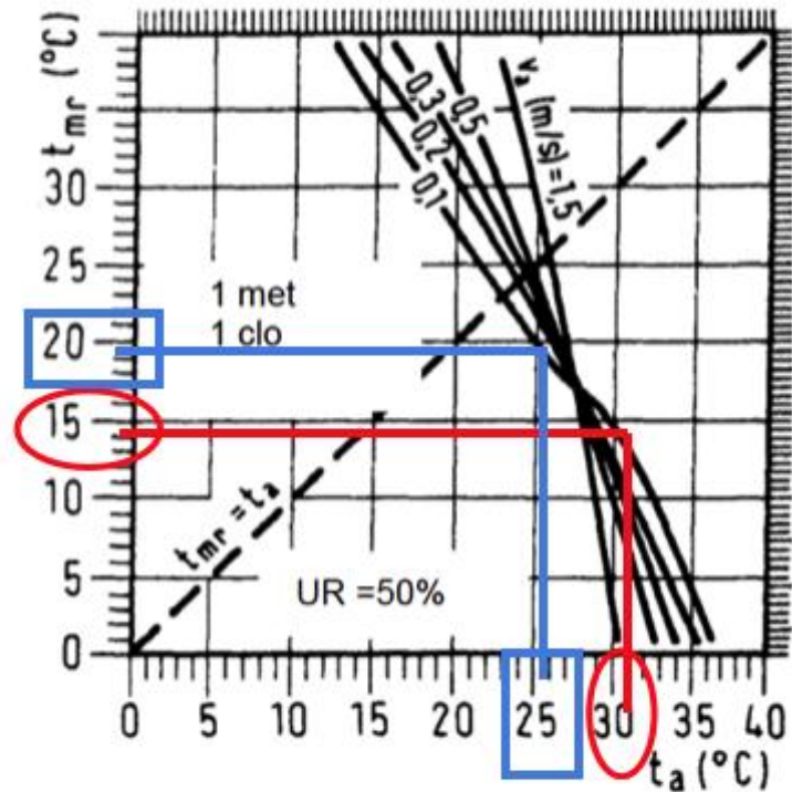
Fig. 3 - Curve isocomfort.
